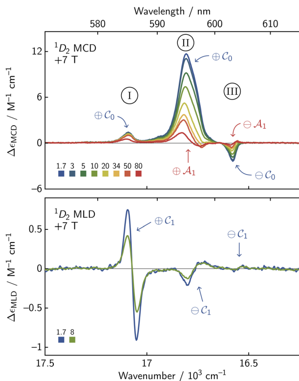
Fig. 5 The MCD and MLD spectra of the three ^3\text{H}_4 \rightarrow ^1\text{D}_2 features in region 2 are labeled with Roman numerals I, II, and III. These features together allow for confident assignment of each transition through comparison of the \overline{\mathcal{C}}_0 , \mathcal{A}_1 , and \mathcal{C}_1 intensities.
