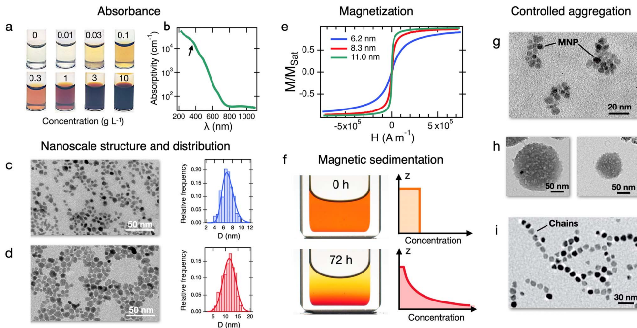
Fig. 1 (a) Dispersions of maghemite ( \gamma - \text{Fe}_2\text{O}_3 ) at concentrations ranging from 0 (pure water) to 10 \text{g L}^{-1} . With increasing concentration, the color evolves from yellow to orange and finally to garnet red at the highest concentration. (b) Mass absorptivity of a \gamma - \text{Fe}_2\text{O}_3 dispersion as a function of wavelength. Data correspond to an 8.3 nm maghemite batch, with concentration independently determined by inductively coupled plasma mass spectrometry. 74 This calibration curve is routinely used to quantify dispersion concentrations. (c and d) TEM images of \gamma - \text{Fe}_2\text{O}_3 nanoparticles with median sizes of 6.2 and 11.0 nm, together with the corresponding size distributions (right panels). (e) Magnetization curves of \gamma - \text{Fe}_2\text{O}_3 dispersions with particle sizes of 6.2, 8.3, and 11.0 nm, normalized to their saturation values. (f) Photographs (left) and concentration profiles (right) of a magnetic dispersion at the initial ( t = 0 h) and final ( t = 72 h) stages of magnetic sedimentation. The magnet is placed at the bottom of the cell, generating a constant magnetic field gradient over the sample height. Fig. 1f is adapted from ref. 45 with permission from the American Chemical Society, copyright 2007. (g and h) MNP aggregates obtained by electrostatic complexation using direct mixing with amphiphilic block-copolymers 75 or a dialysis method, 76 respectively. (i) In situ cryo-TEM images of vitrified magnetite dispersions containing 24 nm iron oxide nanoparticles. Magnetic dipolar interactions lead to anisotropic assemblies including flexible chains, branched chains, and flux-closure rings. The particles shown in this panel were not produced using the Massart synthesis method. Fig. 1i is adapted from ref. 73 with permission from the American Physical Society, copyright 2006.
