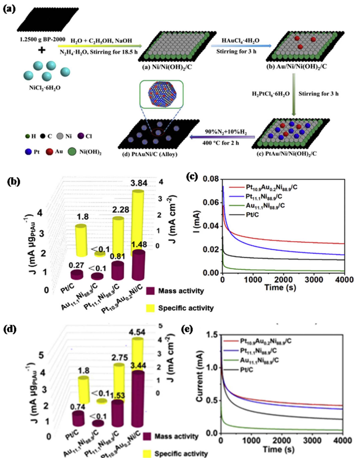
Fig. 5 (a) The systematic route for the synthesis of PtAuNi/C– \text{Pt}_{10.9}\text{Au}_{0.2}\text{Ni}_{88.9}/\text{C} ; (b) MA and SA towards the MOR; (c) chronoamperometry at 0.75 V for the MOR; (d) MA and SA towards the FAOR; (e) chronoamperometry at 0.75 V for the FAOR. This figure has been adapted/reproduced from ref. 160 with permission from Elsevier, copyright 2020.
