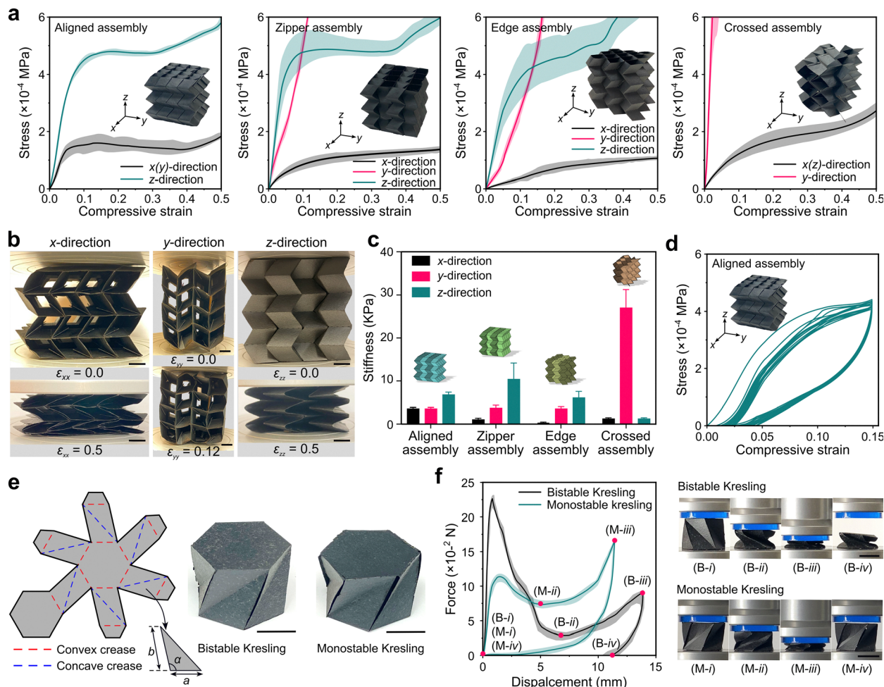
Fig. 4 Mechanical characterization of GO@C/E architected metamaterials. (a) Compressive stress–strain curves of GO Miura-ori architected metamaterials compressed along x-, y-, and z-directions. (b) Digital pictures showing GO@C/E zipper-assembled metamaterials under different compressive strains in x-, y-, and z-directions. The origami can be fully folded in the x- and z-directions but remains stiff in the y-direction. (c) Compressive stiffness of GO@C/E Miura-ori architected metamaterials in different directions. (d) Cyclic (compressive load–unload) responses of aligned assembly; the maximum compressive displacement was 10 mm. (e) Schematic illustration of the Kresling pattern characterized by a , b , and \alpha along with digital pictures of fabricated samples showing the bistable ( a = 13 mm, b = 19.08 mm, and \alpha = 102.77^\circ ) and monostable ( a = 13 mm, b = 17.77 mm, and \alpha = 106.89^\circ ) GO@C/E Kresling origamis. Scale bars: 10 mm. (f) Force–displacement response of bistable and monostable GO@C/E Kresling origamis and digital pictures showing GO@C/E Kresling structures under different compressive displacements. A blue plastic sheet is attached to the surface of the load cell to reduce the friction between the top panel of the GO Kresling and surface of the load cell, enabling its rotation when compressed. B and M denote bistable and monostable designs, respectively. Cyclic (compressive load–unload) responses of Fig. S16(a) bistable GO Kresling and Fig. S16(b) monostable GO Kresling origamis.
