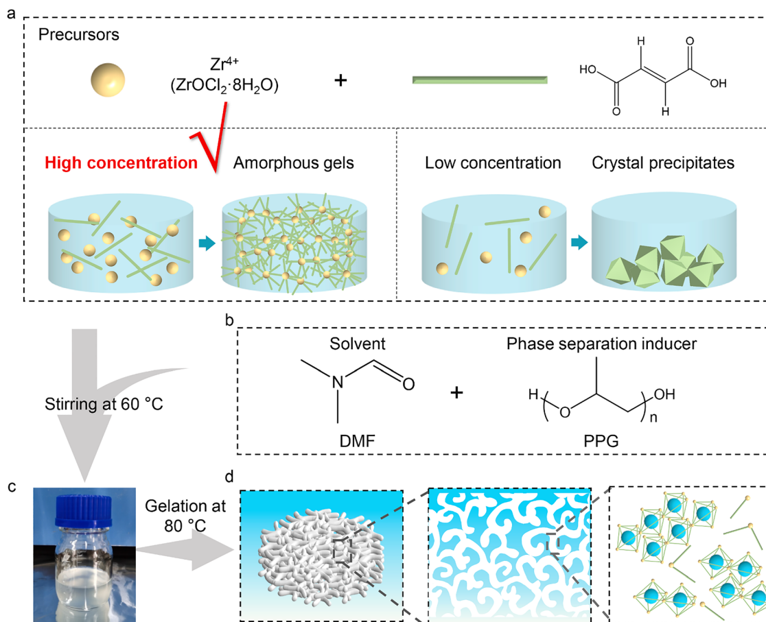
Fig. 3 Schematic of the synthesis of the macroporous MOGs. (a) \text{ZrOCl}_2 \cdot 8\text{H}_2\text{O} and fumaric acid precursors in DMF; (b) introduction of PPG as a phase separation inducer; (c) formation of a homogeneous emulsion after stirring at 60^\circ\text{C} ; (d) formation of macroporous MOGs after gelation at 80^\circ\text{C} accompanied by phase separation. 39 Reproduced from ref. 39. Copyright (2023) Elsevier B. V.
