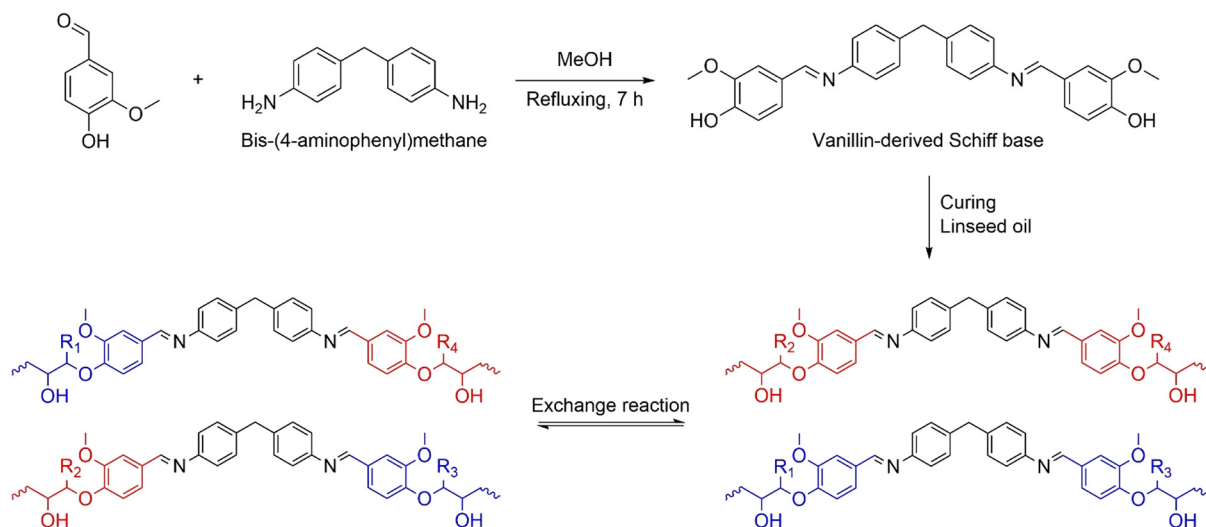
Fig. 10 Scheme of the condensation reaction forming the imine group in a linseed oil-based vitrimer. Adapted from ref. 80 with permission from Elsevier Ltd, Copyright © 2023.
