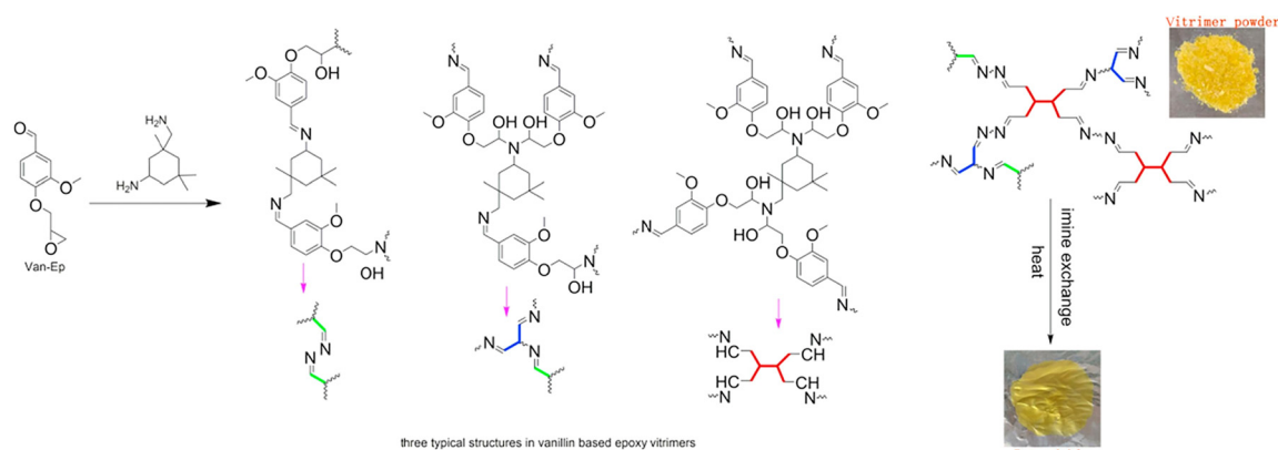
Fig. 12 Epoxidized vanillin–imine exchange reaction in dynamic epoxy networks. Reproduced from ref. 81 with permission from Elsevier Ltd, Copyright © 2019.
