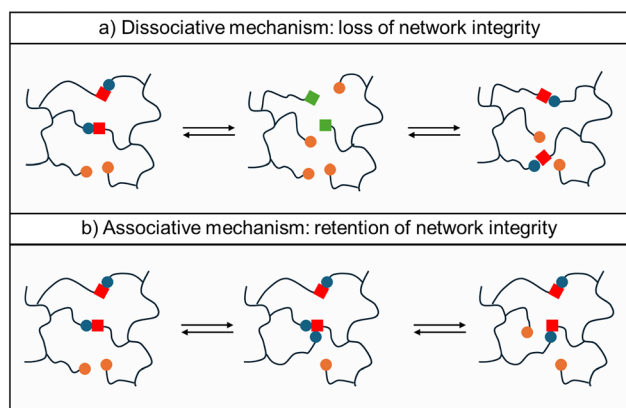
Fig. 3 The two CAN categories: (a) dissociative and (b) associative. In the first case, a loss of network integrity (with a drop in cross-linking density) is observed, while in the second case, there is no loss of network integrity.
