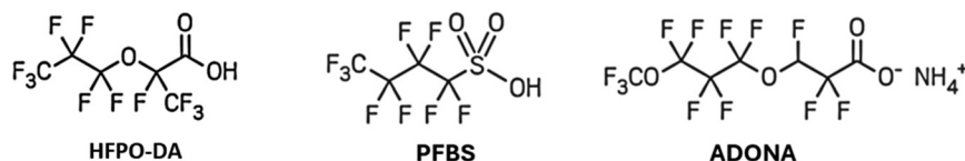
Fig. 1 Structural formula for some legacy PFAS replacements.
