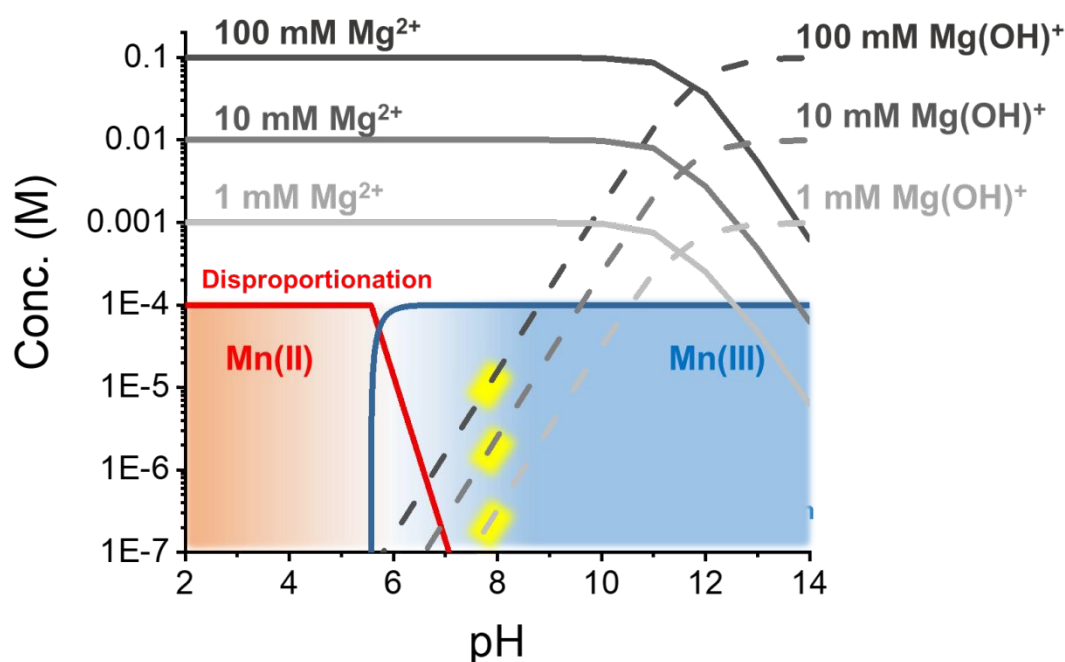
Fig. 3. Thermodynamic equilibrium of disproportionation-comproportionation and \text{Mg}^{2+} aqueous species under varied pH conditions. At pH 7–8, the formation of todorokite closely relates to Mn(III), generated from comproportionation, and to aqueous \text{Mg}(\text{OH})^+ species. The thermodynamic equilibrium of aqueous species in the 1, 10, and 100 mM \text{Mg}^{2+} -added solution with 100 \mu\text{M} \text{Mn}^{2+}(\text{aq}) shows the predominance of Mn(III) and the emerging concentration of \text{Mg}(\text{OH})^+ at pH 7–8. Yellow bold lines indicate the concentration ranges of \text{Mg}(\text{OH})^+ at pH 7–8 in the solutions with 1, 10, and 100 mM. Based on the oxidation rates of \text{Mn}^{2+}(\text{aq}) with superoxide ( \leq \sim 3.3 \mu\text{M}/\text{h} ), the concentration of Mn(III), generated from comproportionation, is comparable to that of \text{Mg}(\text{OH})^+ in the solutions with 10 and 100 mM \text{Mg}^{2+} . The concentrations of \text{Mg}(\text{OH})^+ in the solutions with 10 and 100 mM \text{Mg}^{2+} are orders of magnitude higher than that of \text{Mg}(\text{OH})^+ in the solution with 1 mM \text{Mg}^{2+} . The figure information is generated from thermodynamic calculations using Visual MINTEQ and the thermo.vdh thermodynamic database. The equilibrium
