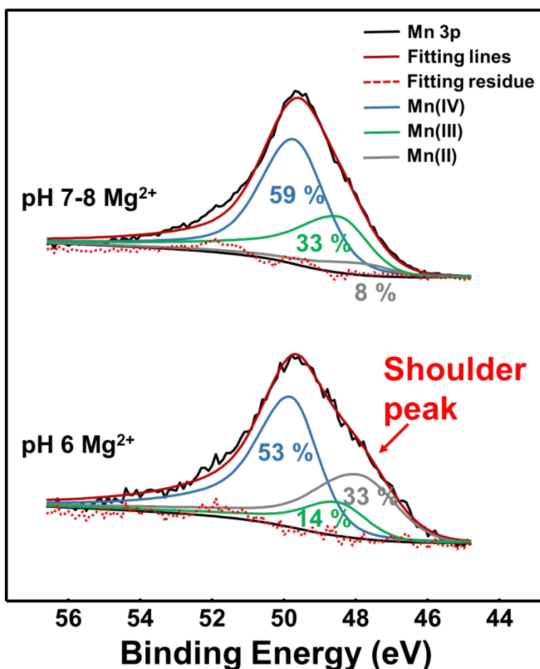
Fig. 2. Predominance of Mn(III) over Mn(II) in Mn oxides prepared at pH 7–8. Although Mn(IV) is the most dominant oxidation state in all reaction systems, analyses of X-ray photoelectron spectroscopy of Mn3p show that the dominance of Mn(III) or Mn(II) changes depending on the pH condition. The fitting lines of Mn(II), Mn(III), and Mn(IV) are in gray, green, and blue, respectively. At pH 6, a significant extent of Mn(II) occurs at the shoulder peak at around 47.8 eV. This discrepancy in the oxidation state results from the equilibrium of comproportionation-disproportionation reactions, depending on the pH condition.
