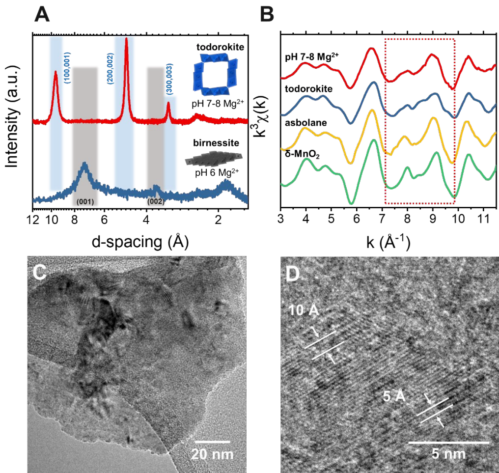
Fig. 1. The formation of todorokite at pH 7–8 in the presence of Mg 2+ . (A) X-ray diffraction of Mn oxides shows the clear diffractions of todorokite (blue bar) at pH 7–8. At pH 6, only birnessite (or δ-MnO 2 ) was observed after 6 h reaction. (B) The analysis of extended X-ray absorption fine structure supports the formation of todorokite at pH 7–8. TEM images of the platy show the morphology of poorly crystalline todorokite (C) and the large d-spacing of todorokite (D) prepared at 100 mM Mg 2+ pH 7–8.
