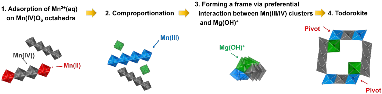
Fig. 4. Schematic illustration of the direct formation mechanism of todorokite via the oxidation of \text{Mn}^{2+}(\text{aq}) with superoxide in the presence of \text{Mg}^{2+} under circumneutral conditions. Edge-sharing Mn(III) clusters occur from comproportionation between \text{Mn}^{2+}(\text{aq}) and \text{Mn(IV)O}_6 octahedra (Stages 1 and 2). Edge-sharing Mn(IV) and Mn(III) clusters in solution interact with \text{MgOH}^+ and form a framework element of todorokite (Stage 3). Further assembly forms todorokite by conforming the frame (Stage 4).
