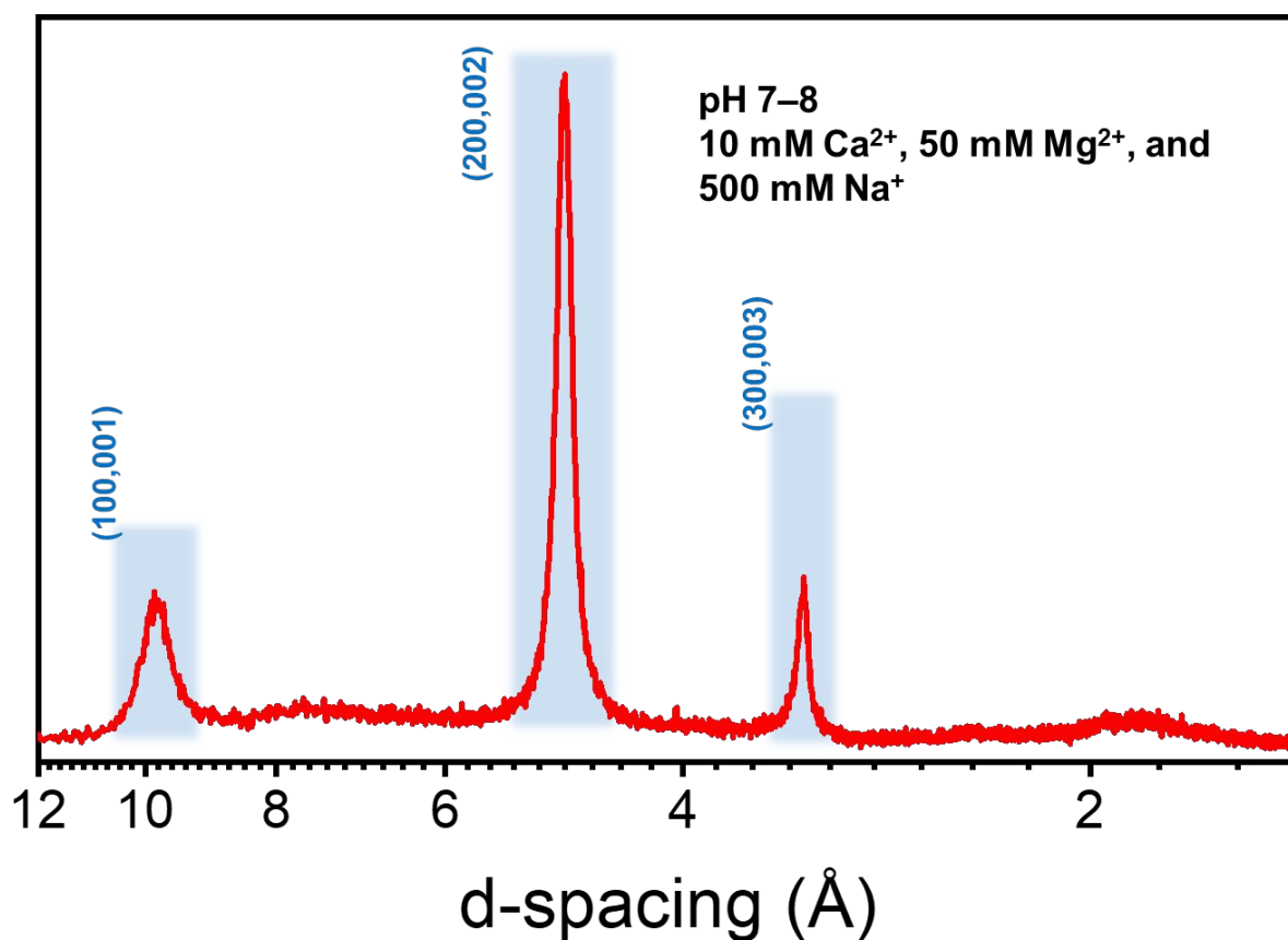
Fig. 5. The formation of todorokite in the presence of multiple cations. Although the concentrations of Mg 2+ and Ca 2+ are much lower than that of Na + in the seawater mimicked solution, the XRD result shows the formation of todorokite, suggesting the feasibility of the reaction in environmental systems.
