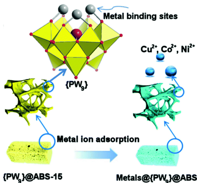
Fig. 7 Schematic illustration of the POM-modified 3D-printed copolymer substrates used for transition-metal removal by the cation binding sites of the lacunary [α-PW 9 O 34 ] 9- . Reproduced from ref. 205 with permission from The Royal Society of Chemistry, copyright 2018.
