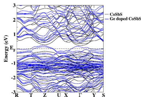
Fig. 3 Electronic band structures of CoSbS (black) and Ge-substituted \text{Co}(\text{Sb}_{0.875}\text{Ge}_{0.125})\text{S} (blue). Reproduced with permission from The Royal Society of Chemistry ©2024 (License CC BY 3.0). 220
