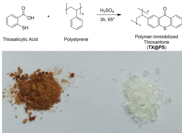
Scheme 1 (Top) In situ formation of TX moieties by reaction of polystyrene and thiosalicylic acid in the presence of sulfuric acid (H 2 SO 4 ), yielding TX@PS; (bottom) photograph of TX@PS (left) and polystyrene (right).
