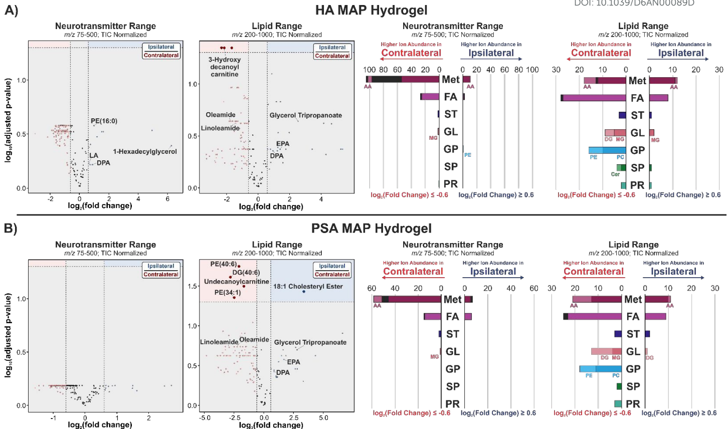
Figure 5. Volcano plots and summary bar charts for two mass ranges m/z 75-500 and m/z 200-1000 for both hydrogel-treated samples: (A) HA MAP hydrogel and (B) PSA MAP hydrogel. The volcano plots compare the \log_2(\text{fold change}) between the ipsilateral (lesion) region and contralateral (healthy) region of the brain. These regions consist of the infarct and per-infarct region of the brain (lesion) and a similar sized region of interest (ROI) from the contralateral side of the brain. The size of ROIs corresponds to the sample/replicate and varies accordingly to account for only the affected area and the opposite hemisphere of the brain. All p-values were adjusted according to a Benjamini-Hochberg correction with a cutoff of -\log_{10}(\text{p-value}) = 1.3 (p-value of 0.05). Key metabolites and lipids of interest are labeled accordingly according to tentative annotations in Table S2 . The summary bar charts account for all polar metabolites and lipid categories impacted with respect to the \log_2(\text{fold change}) . All -\log_{10}(\text{Benjamini-Hochberg corrected p-values}) and \log_2(\text{fold changes}) are included in Table S2 . Additional comparisons between the ipsi- and contralateral regions of the brain between HA-MAP and PSA-MAP are found in Figure S5 and resulted in no statistically significant differences.
