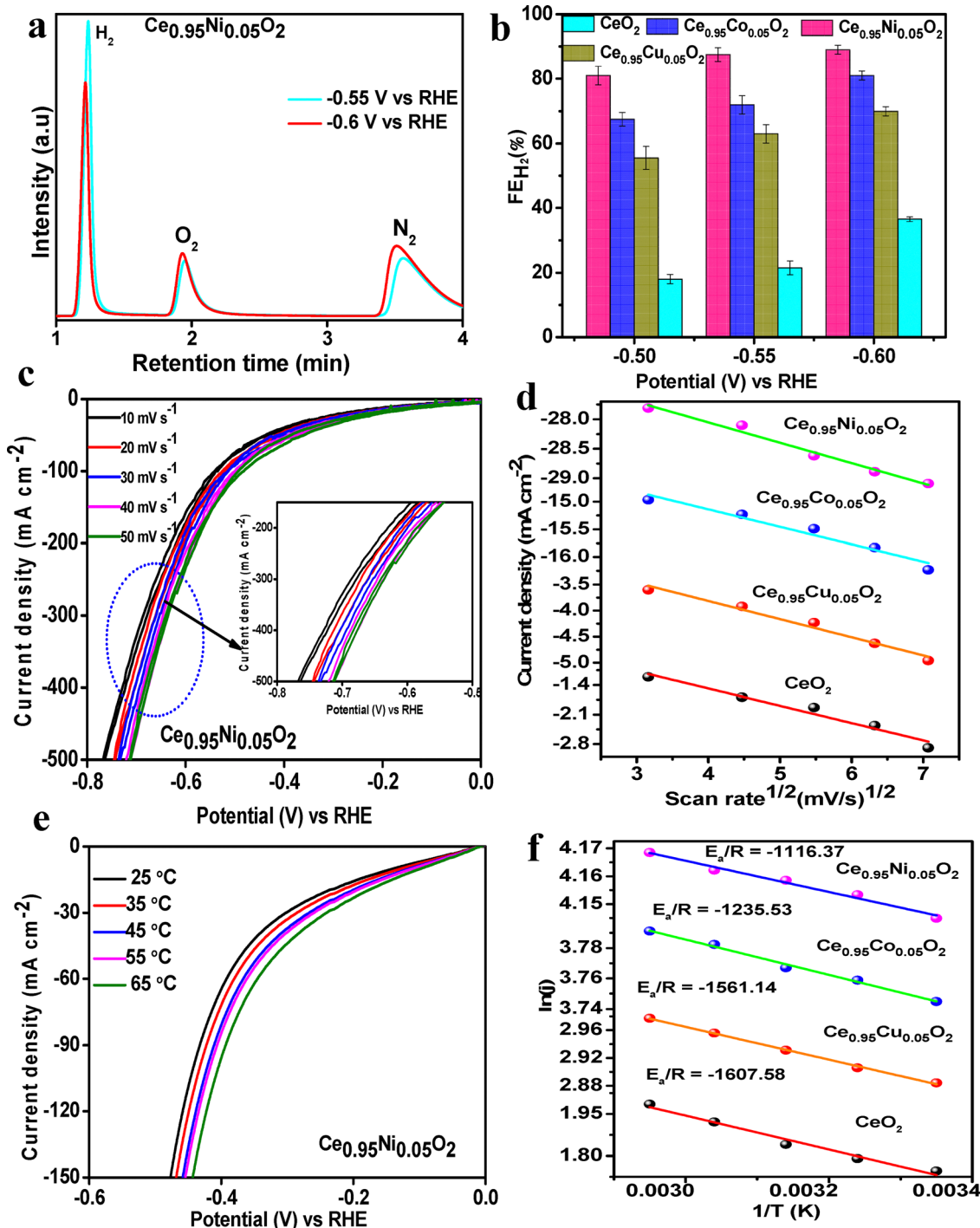
Fig. 7 (a) Representative GC chromatograms of \text{H}_2 from \text{Ce}_{0.95}\text{Ni}_{0.05}\text{O}_2 after 1 h of chronoamperometric study; (b) \text{FE}_{\text{H}_2} of the four catalysts at varied potentials; (c) CV of \text{Ce}_{0.95}\text{Ni}_{0.05}\text{O}_2 with different scan rates; (d) scan rate-dependent study of the four catalysts; (e) LSV of \text{Ce}_{0.95}\text{Ni}_{0.05}\text{O}_2 at various temperatures and (f) activation energy plot of the hydrogen evolution reaction over the four synthesized materials.
