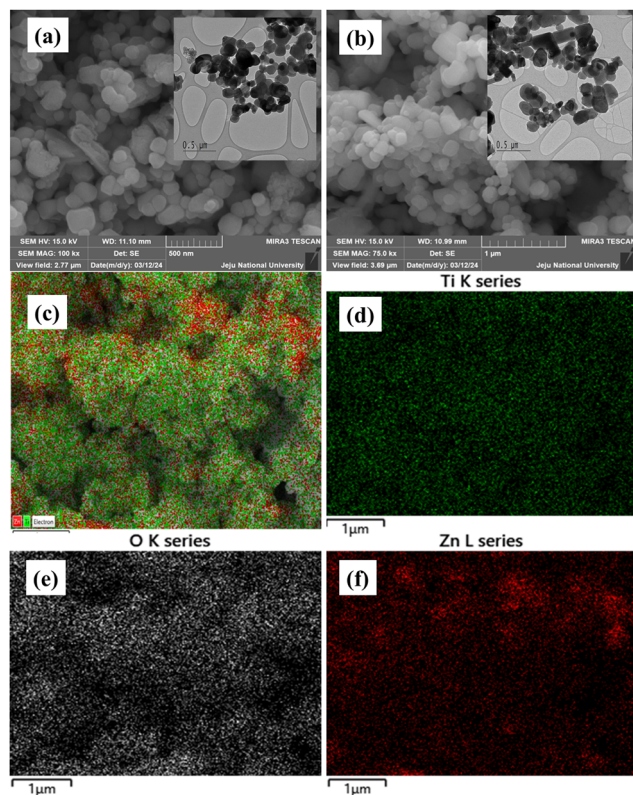
Fig. 6 FESEM images of (a) bare \text{TiO}_2 NPs, (b) TZ-3 NCs, and (c) elemental mapping of TZ-3 NCs representing element Ti (d), O (e), and Zn (f).
