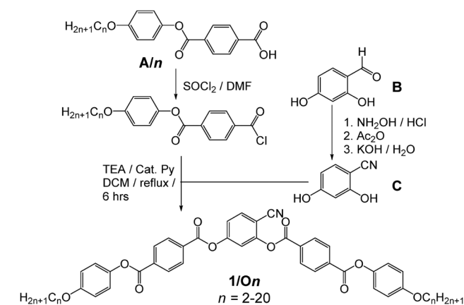
Scheme 1 Synthetic route to the bent-core mesogens 1/On .
