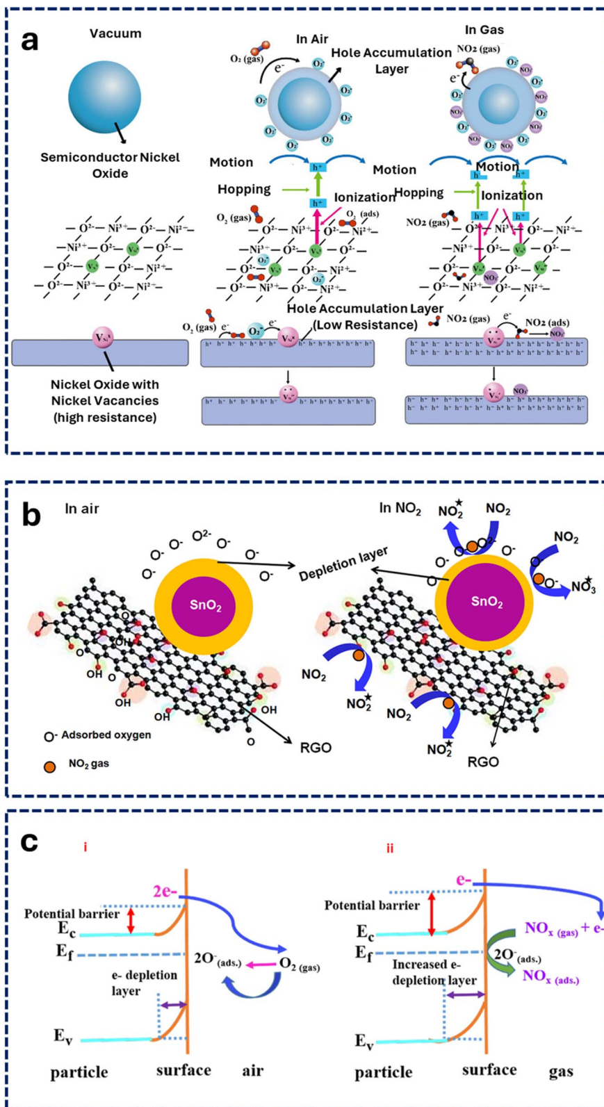
Fig. 13 Gas sensing mechanisms: NiO, SnO 2 /RGO, and Pd@V 2 O 5 sensor diagram. (a) NiO-Ni 0.9 O sensor system in a vacuum, air, and NO 2 at room temperature (RT) (reprinted with permission, 182 Copyright 2024, American Chemical Society); (b) gas sensing mechanism diagram of the SnO 2 /RGO sensor for NO 2 gas (reprinted with permission, 183 Copyright 2021, Elsevier); (c) schematic representation of the sensing mechanism of 1 wt% Pd@V 2 O 5 towards (i) air and (ii) NO x (reprinted with permission, 177 Copyright 2020, Elsevier).
