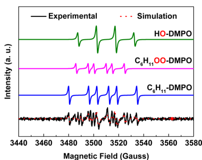
Fig. 8 Quenching experiments (a) and EPR measurements (b) of cyclohexane oxidation with O 2 irradiated under visible light utilizing T(4-COOH)PP as the photocatalyst.
