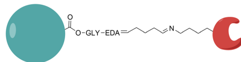
Scheme 9 Schematic illustration of the different functionalized immobilization carriers using the NHS-ester activated PASP (carrier I: PASP-EDC/NHS), the NHS-ester activated and ethylenediamine/glutaraldehyde functionalized PASP (carrier II: PASP-EDA-GLU), as well as the glycidol activated and ethylenediamine/glutaraldehyde functionalized PASP (carrier III: PASP-GLY-EDA-GLU) for the immobilization of CalB.
