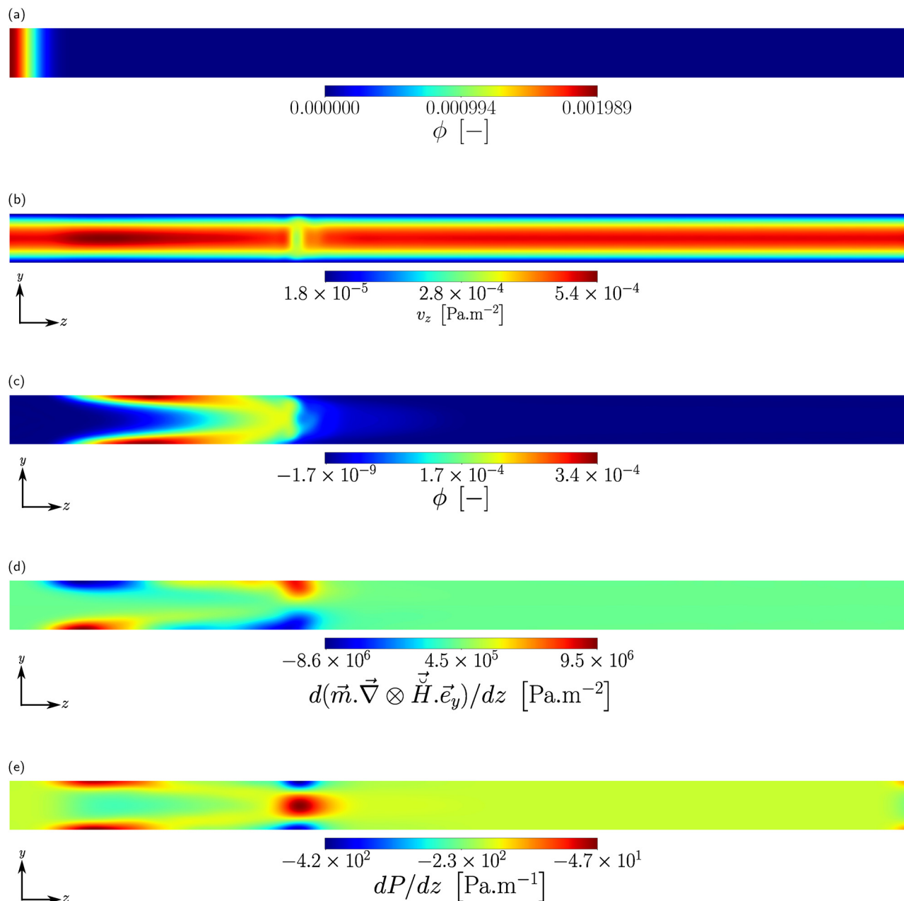
Fig. 6 Initial condition and flow/MNP distribution in the yz -plane under an SMF ( \alpha = 1 , H_0 = 14.713 kA m -1 ): (a) prescribed Gaussian concentration profile at the inlet ( z = 0 ), used as the initial condition for the MNP pulse; (b) axial velocity at t = 10 s; (c) MNP concentration at t = 10 s; (d) axial variation of the transverse Kelvin body force at t = 10 s; and (e) axial pressure gradient at t = 10 s. Parameters: v_0 = 0.25 mm s -1 ( Pe \approx 1145 , Re \approx 0.05 ); injected concentration \phi_0 = 5 \times 10^{-5} ; particle diameter D_p = 10 nm; domain magnetization M_d = 425 kA m -1 .
