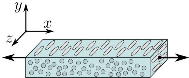
Fig. 2 Geometry and alignment of LCEs in this study. The nematic director in the unstrained LCEs is along the z-axis, strain is applied along the x-axis. The thickness of the LCE, i.e. the dimension in which the auxetic response is observed, is along the y-axis.
