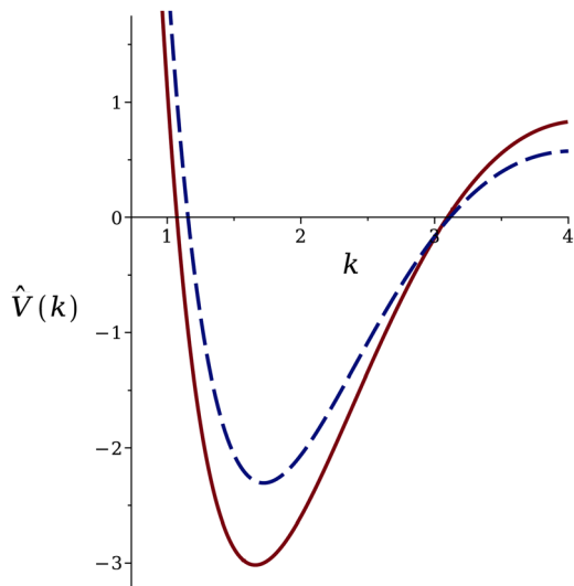
Fig. 2 The interaction potential times the pair distribution function in Fourier representation, \hat{V}(k) . Red solid line: u_{hs} = u_{hs}^+ (hard spheres). Blue dashed line: u_{hs} = u_{hs}^s (eqn (4), nearly hard spheres) k is in \sigma^{-1} units, and \hat{V}(k) is in arbitrary \epsilon units.
