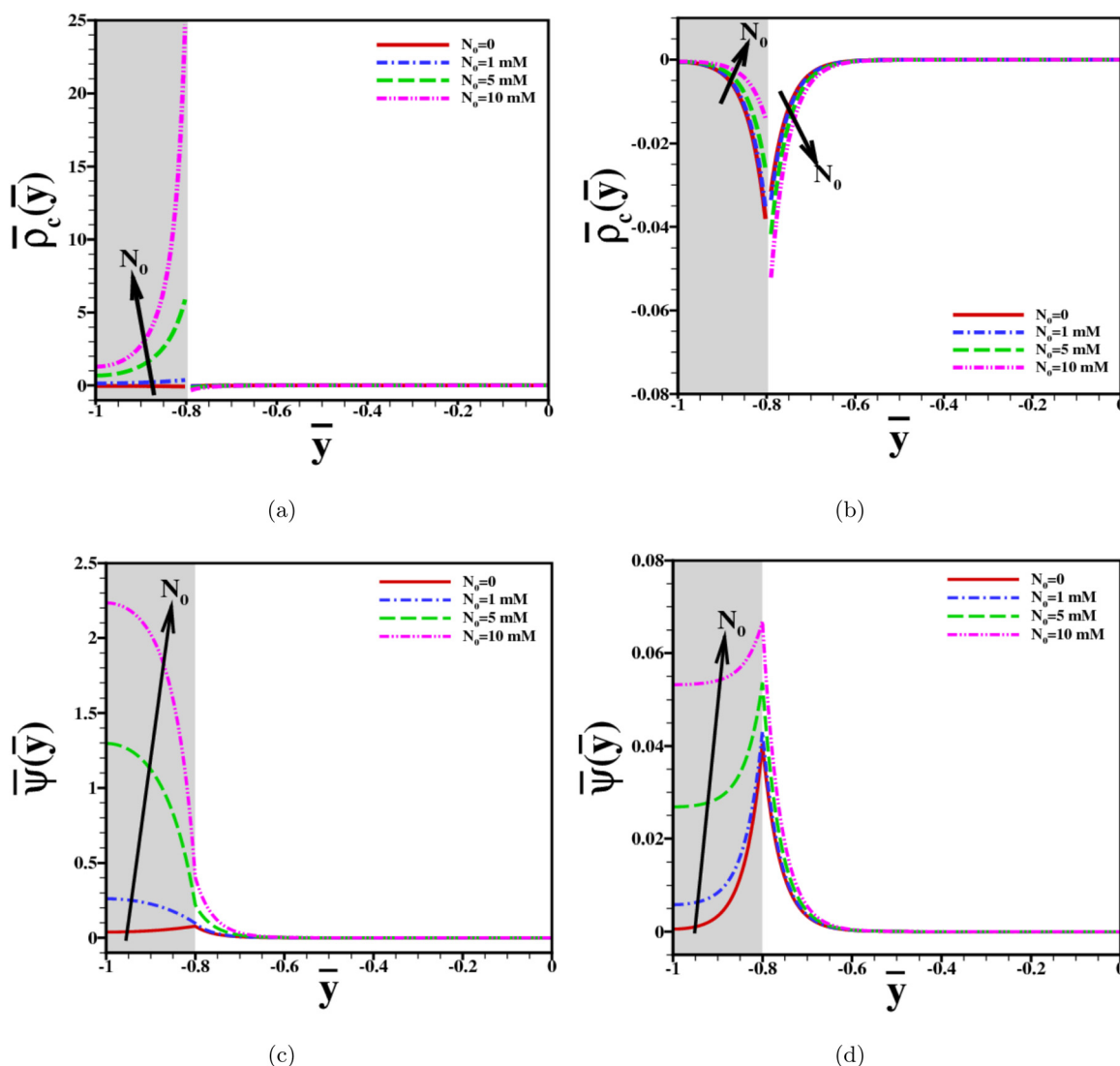
Fig. 17 Charge distribution of mobile ions \bar{\rho}_c(\bar{y}) (in the scaled form) and scaled potential distributions \bar{\psi}(\bar{y}) are shown as a function of scaled spatial coordinate \bar{y} for various values of N_0 (0, 1 mM, 5 mM, and 10 mM). In (a) and (c) we consider \epsilon_R = 0.1 and in (b) and (d) the value of dielectric permittivity ratio \epsilon_R = 1 . Other model parameters are H = 25 nm, \delta = 5 nm, \kappa H = 25 , \bar{\sigma} = 2 , and r = 3.3 Å, respectively.
