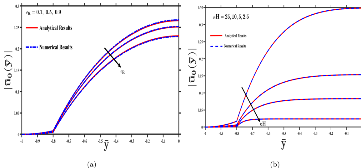
Fig. 14 In Fig. (a) and (b) we have shown the scaled velocity amplitude |u_0(\bar{y})| as a function of \bar{y} for various values of \epsilon_R ( = 0.1, 0.5 , and 0.9 ) with fixed \kappa H = 2.5 ; and various values of \kappa H ( = 2.5, 5, 10 , and 25 ) with fixed \epsilon_R = 0.1 . Other model parameters are H = 25 nm, \delta = 5 nm, N_0 = 1 mM, \rho_R = 1.35 , \eta_R = 2.54 , \bar{\sigma} = 1 and \bar{\omega} = 10 , respectively.
