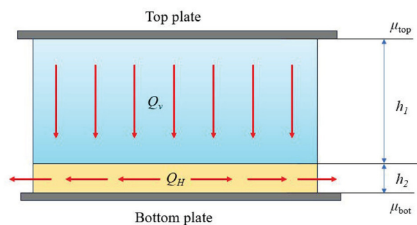
Fig. 5 (a) Fluid outflow from the sample visualized by colored liquid. A fibrin gel at a concentration of 15\text{ mg ml}^{-1} was polymerized with a blue stained buffer. After compression the colored fluid leaves the sample only from the bottom over a period of minutes. (b) Schematic representation of fluid flow in our compressed gel samples. The flow in the upper layer (height h_1 ) is directed downward, while the flow in the lower layer (height h_2 ) is radial. The chemical potential at the middle of the top plate is denoted by \mu_{\text{top}} and that at the middle of the bottom plate \mu_{\text{bot}} . The lower layer thickness h_2 is significantly smaller than the upper layer thickness h_1 ( h_2 \ll h_1 ). These two layers are not to be confused with densified and rarefied phases that are formed under compression.
