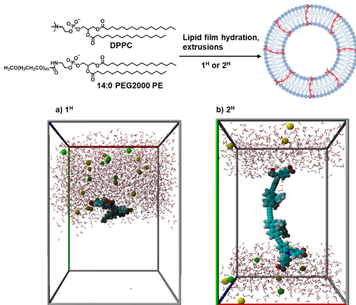
Fig. 7 Integration of 1^{\text{H}} or 2^{\text{H}} into a DPPC (1,2-dipalmitoyl- sn -glycero-3-phosphocholine) liposome and a molecular dynamic simulation snapshot of (a) 1^{\text{H}} and (b) 2^{\text{H}} in DPPC after 100 ns simulation time. The lipid bilayer membrane is omitted for clarity.
