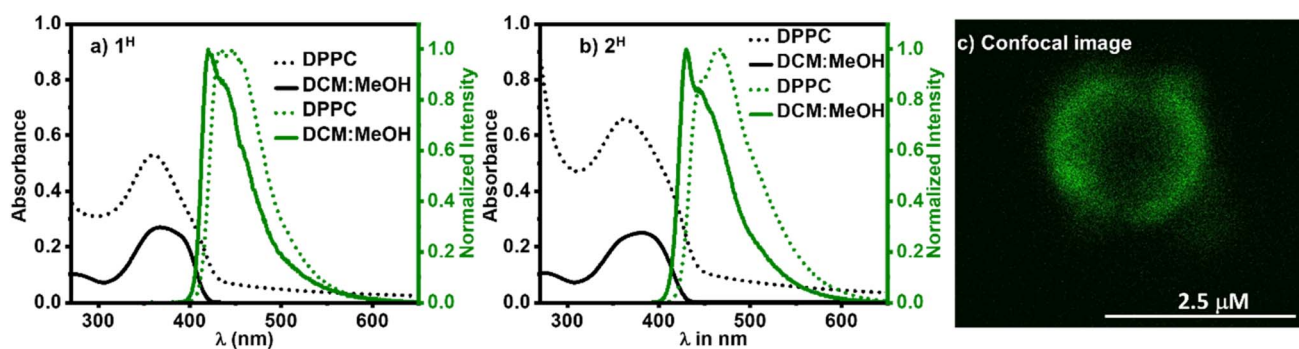
Fig. 8 (a) UV-Vis and emission spectra of 1^{\text{H}} and (b) UV-Vis and emission spectra of 2^{\text{H}} in a mixture of dichloromethane (DCM) : methanol (MeOH) (1 : 1) and in DPPC liposomes with a composition of DPPC : (14:0 PEG2000 PE) : 1^{\text{H}} or 2^{\text{H}} = 100 : 1 : 1, in phosphate buffer at pH = 7.0; (c) confocal microscopy image of 2^{\text{H}} in a giant vesicle with a composition of 100 : 1 : 1 of DPPC : 14:0 PEG2000PE : 2^{\text{H}} in phosphate buffer at pH = 7.0 after size exclusion chromatography, upon fixation in agarose hydrogel.
