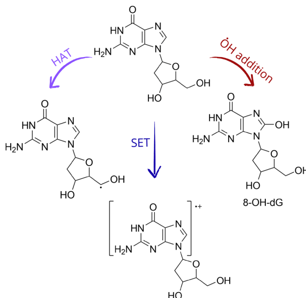
Scheme 4 Some of the most relevant oxidation products of 2'-deoxyguanosine (2dG).
