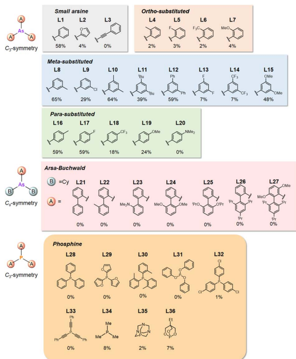
Fig. 2 o -, m -, and p -substituted C_{3-} and C_{2-} -type arsinic and phosphinic ligands. The NMR yield of the difunctionalized product 1 (Scheme 1) is shown below each structure.
