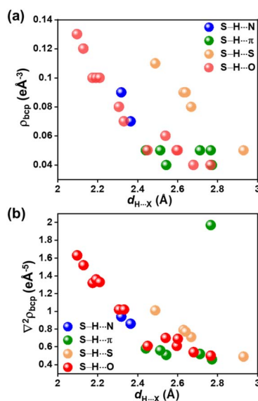
Fig. 5 Correlation plots of (a) electron density ( \rho_{\text{bcp}} ) and its (b) Laplacian ( \nabla^2 \rho_{\text{bcp}} ) with interaction distances ( d_{\text{H}\cdots\text{X}} ) of various S–H \cdots X interactions from our HAR models.
