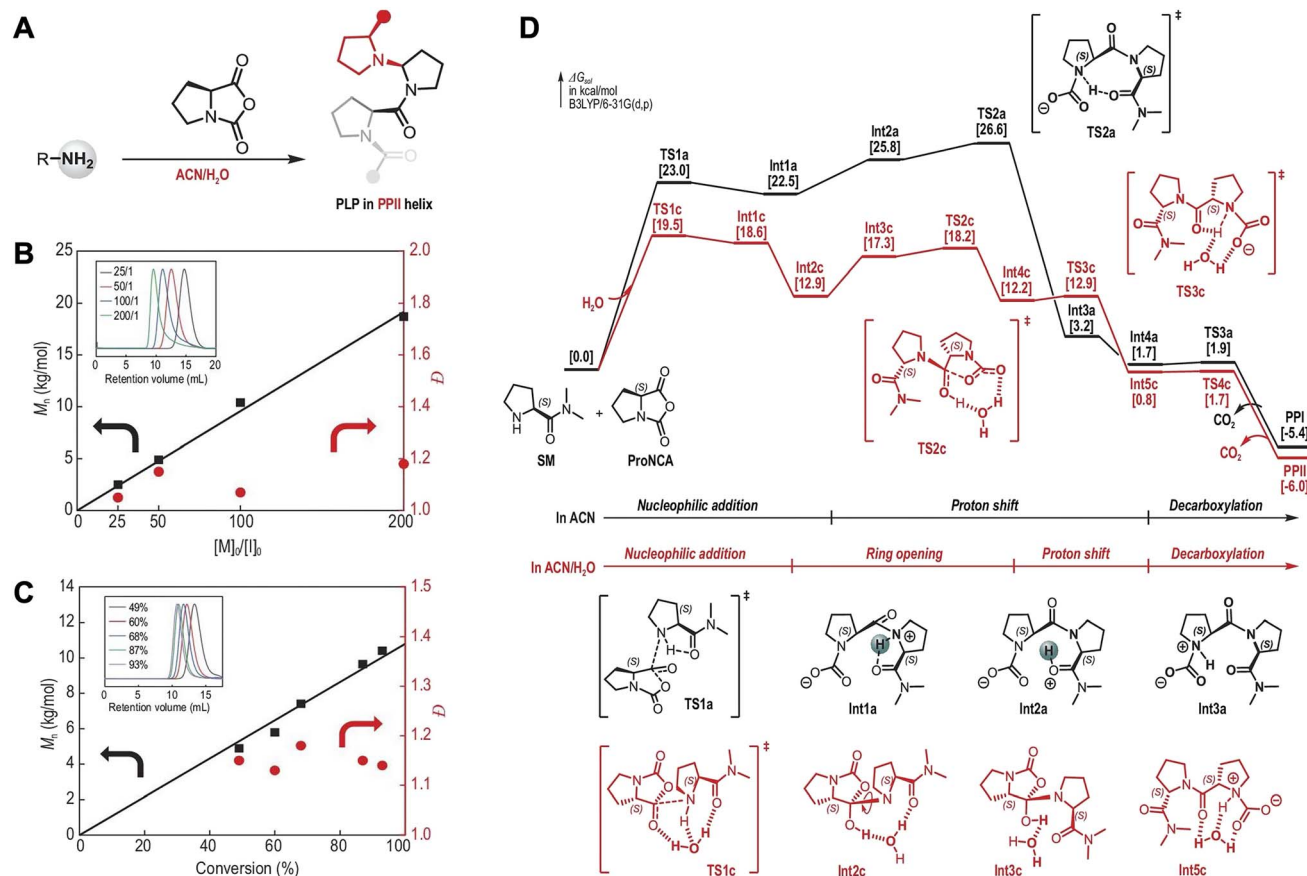
Fig. 7 (A) ROP of Pro-NCA in mixed acetonitrile/H 2 O; (B) M_n and \bar{D} of polyproline as a function of [\text{Pro-NCA}]_0/[\text{I}]_0 ratio; (C) conversion of Pro NCA ( [\text{Pro-NCA}]_0/[\text{I}]_0 = 100/1 ); (D) plausible pathways for the ROP of Pro-NCA in dry acetonitrile (black) and mixed acetonitrile/H 2 O (red) revealed by density functional theory (DFT) calculations. Reproduced with permission from ref. 52. Copyright 2022, Oxford University Press.
