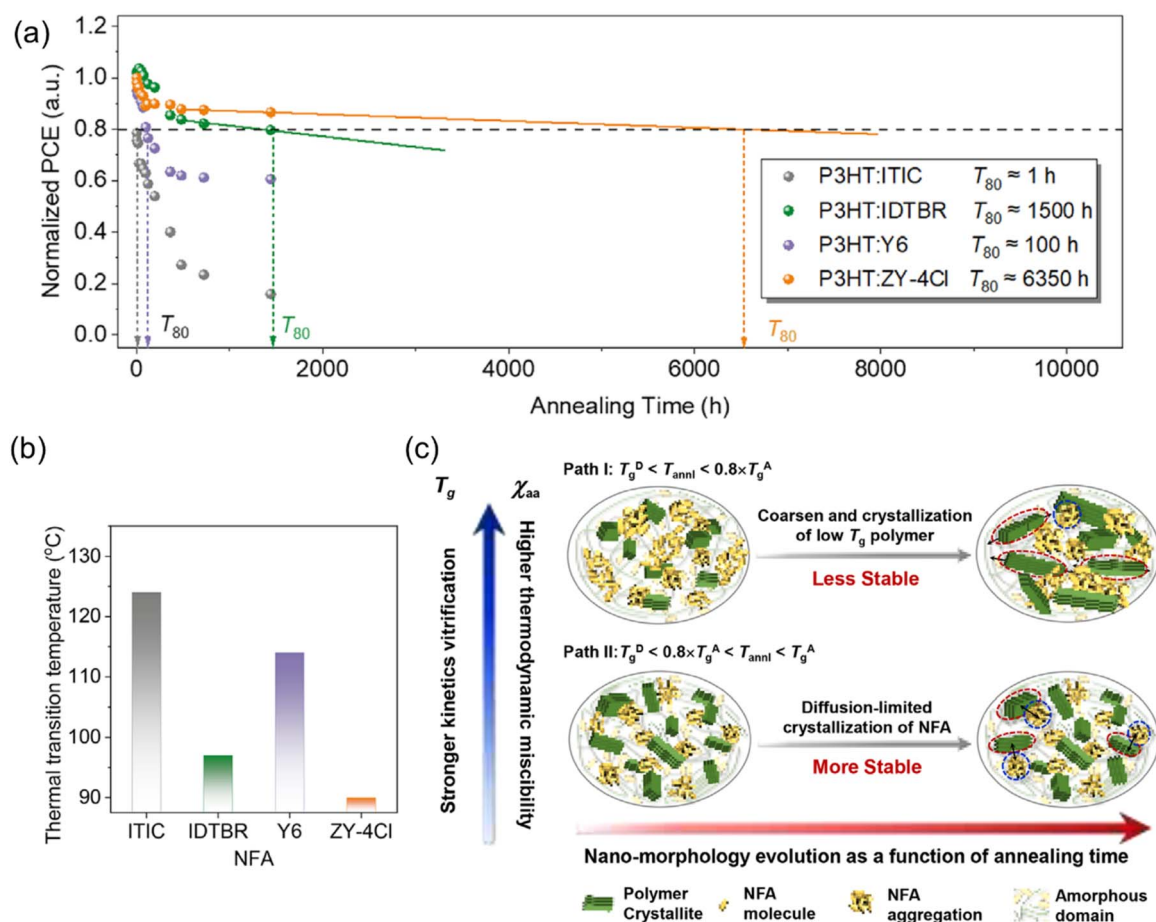
Fig. 14 (a) Normalized power conversion efficiencies (PCEs) of the four P3HT:NFA devices versus the annealing time of the active layer under continuous thermal heating at 80 °C. (b) The plot of the thermal transition temperatures ( T_g ) of the four nonfullerene acceptors. (c) Schematic illustrations of two paths of nanomorphology evolution as a function of time. In this work, P3HT:ITIC ( T_g^D ( T_g of the crystalline polymer donor) < T_{annl} < 0.8 \times T_g^A ( T_g of the small molecule acceptor)) and P3HT:ZY-4Cl ( T_g^D < 0.8 \times T_g^A < T_{annl} < T_g^A ) belong to the typical cases of paths I and II, respectively. 112
