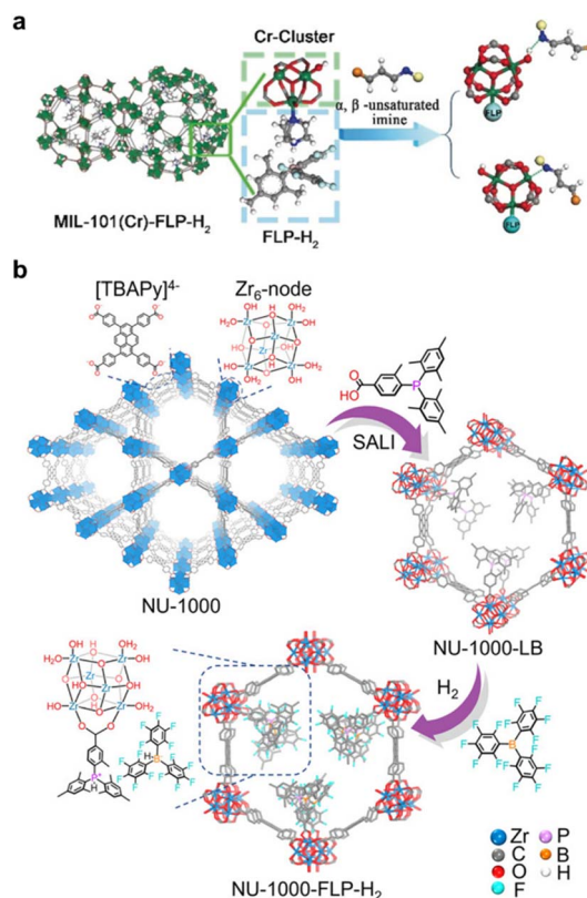
Fig. 13 (a) The "activation" process involving a \text{Cr}_3(\mu_3\text{-O})(\text{COO})_6(-\text{OH})(\text{H}_2\text{O})_2 cluster in MIL-101(Cr)-FLP-H 2 . Reproduced with permission. 219 Copyright 2019, John Wiley and Sons. (b) Construction pathway of NU-1000-FLP-H 2 . Reproduced with permission. 220 Copyright 2023, American Chemical Society.
