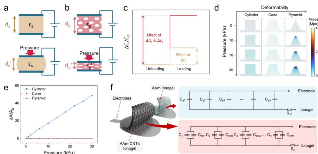
Fig. 5 Schematic illustration of (a) a capacitive pressure sensor using a solid elastomeric dielectric layer, (b) a piezocapacitive pressure sensor using a porous elastomeric dielectric layer, and (c) capacitance changes in solid and porous elastomeric dielectric layer-based pressure sensors induced by identical loading. Reproduced with permission. 199 Copyright 2016, American Chemical Society. (d) Results of finite element analysis of the stress distribution for different architectures (cylinder, cone, and pyramid) under varying pressures, (e) profiles of the contact area of microstructure electrode/electrolyte interfaces vs. applied pressures, and (f) the equivalent circuit of two ICPSs. Reproduced with permission. 27 Copyright 2023, American Chemical Society.
