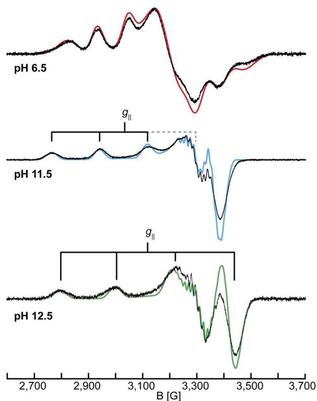
Fig. 2 CW X-band (9.46 GHz) EPR spectra of SmAA10A at pH 6.5, 11.5 and 12.5 in black with EPR simulations in color. The simulation for pH 12.5 uses the 14 N couplings of case A (see section on 14 N ENDOR). EPR parameters are listed in Tables 1 and S1† and experimental conditions are reported in the Experimental section.
