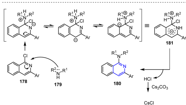
Scheme 47 Sonochemical synthesis of 1-aminoisoquinoline derivatives 180 through the reaction of 1-chloroisoquinoline 178 with appropriate amines 179 .
