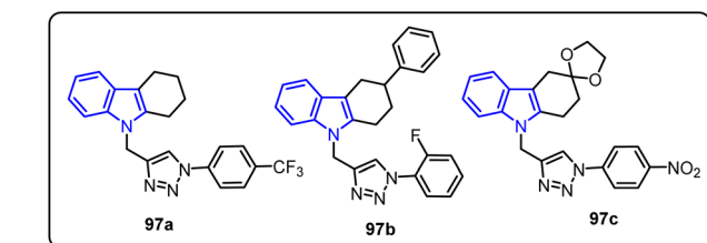
Scheme 22 Synthetic pathway for the preparation of novel indole-substituted functionalized 1,2,3-triazole-based carbazole derivatives 97 .
