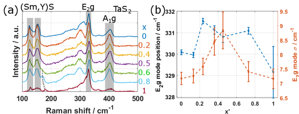
Fig. 8 Raman analysis of the specimens. (a) Comparison of Raman spectra obtained by averaging three spectra from different NTs for each value of x . The RSI and II modes of the (\text{Sm}, \text{Y})\text{S} subsystem, an additional peak for small values of x (dotted gray line) and the E_{2g} and A_{1g} modes of \text{TaS}_2 are resolved. The spectrum for x = 0 was acquired in a different instrument and with a different objective. (b) Plot of the E_{2g} mode position and E_{2g} mode width \sigma in dependence of x' .
