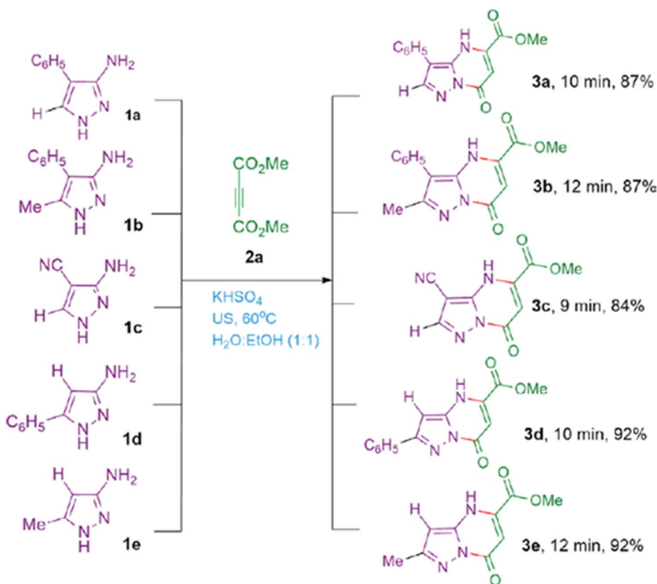
Scheme 20 Synthesis of 2 or/and 3-substituted methyl 7-oxo-4,7-dihydro-5H-pyrazolo[1,5- a ]pyrimidine-5-carboxylate. 106
