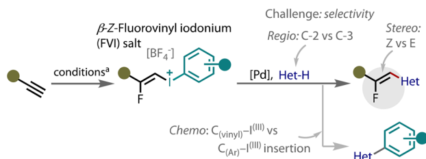
[C] Our strategy: \beta -Fluorovinylolation from alkynes via FVI salts
