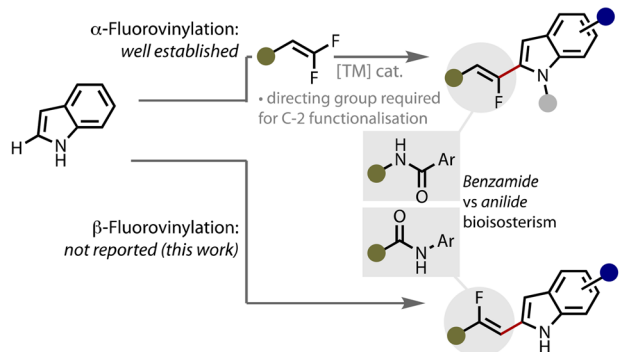
[C] Our strategy: \beta -Fluorovinylolation from alkynes via FVI salts
