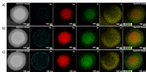
Fig. 21 Electron image, elemental mapping images, and EDX layered images of (a) \text{Fe}_3\text{O}_4@MIL-100(\text{Fe})\text{-Pt}(10) , (b) \text{Fe}_3\text{O}_4@MIL-100(\text{Fe})\text{-Pt}(20) , and (c) \text{Fe}_3\text{O}_4@MIL-100(\text{Fe})\text{-Pt}(30) . Adapted with permission from ref. 52. Copyright 2020 American Chemical Society.
