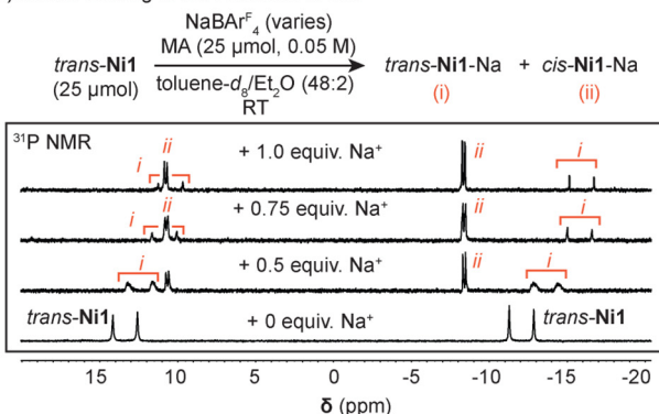
Fig. 1 Addition of M^+ to Ni1 leads to the formation of cis and trans Ni1 -M species in solution (A). 31 P NMR spectra (202 MHz) of Ni1 after the addition of up to 1.0 equiv. of NaBAR^F_4 in the absence (B) and presence (C) of MA. Ar = 2-methoxyphenyl.
