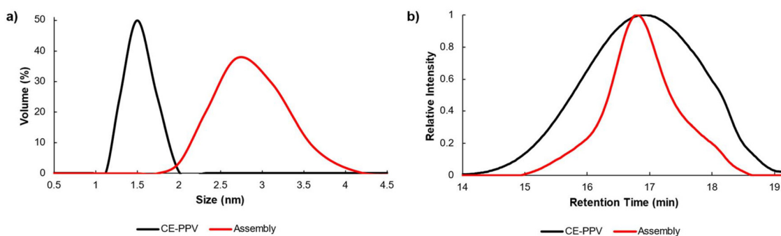
Fig. 3 (a) DLS in 1 : 1 CHCl 3 /CH 3 CN and (b) GPC characterization in THF, against linear PS standards, of homopolymer CE-PPV ( 13b ) (black) and the supramolecular bottlebrush CE-PPV-PS-DBA + (red).
