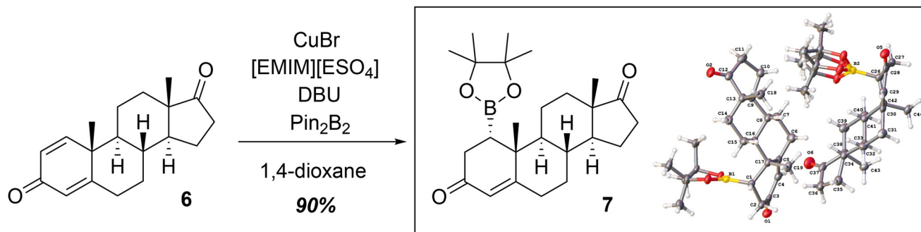
Scheme 1 Successful 1,4-borylation of androst-1,4-dien-3,17-dione (6) to yield borane adduct 7. [EMIM][ESO 4 ]: 1-ethyl-3-methylimidazolium ethyl sulfate (Step 1 of 8 steps).
