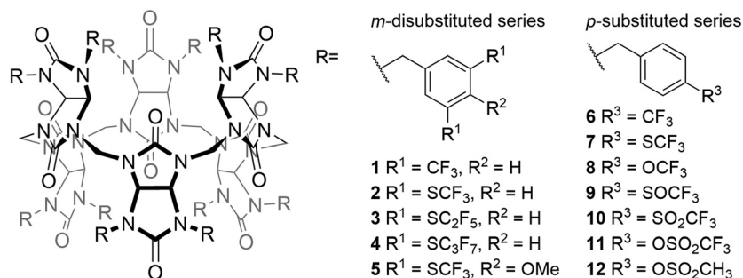
Fig. 1 Structures of the investigated bambusurils.
