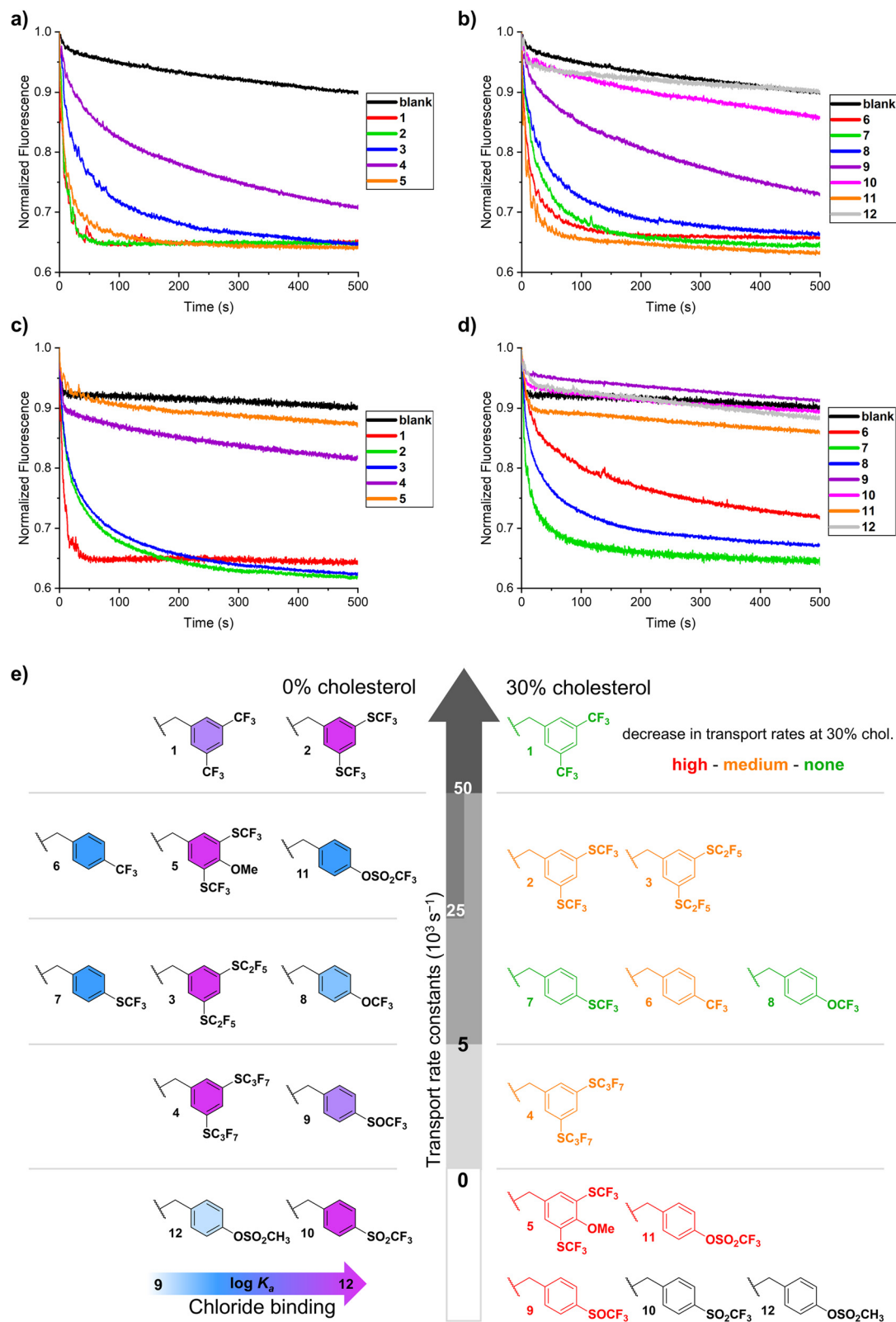
Fig. 5 The transport of chloride via \text{Cl}^-/\text{HCO}_3^- antiport by BUs (pre-incorporated at 0.02 mol%) monitored by the lucigenin assay in 225 mM \text{NaHCO}_3 , upon addition of 25 mM NaCl to LUVs composed of either POPC only (a and b), or POPC/cholesterol 7:3 (c and d); control experiments without any BU are indicated as 'blank'; (e) graphical visualization of the anion transport rate constants at 0% (left part) and 30% (right part) cholesterol content in the membrane, with the binding strength to chloride indicated in the left part (light blue = the weakest binding, purple = the strongest binding) and the effect of cholesterol on transport rates indicated in the right panel (red = transport stopped, orange = transport decreased, green = no significant effect).
