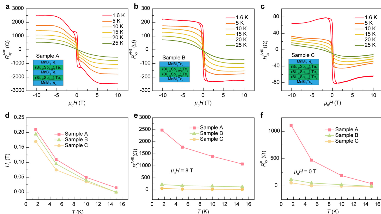
Fig. 4 Temperature-dependent anomalous Hall resistance in (\text{Bi}_{0.56}\text{Sb}_{0.44})_2\text{Te}_3 -intercalated \text{MnBi}_2\text{Te}_4 multilayers with different spacer layer thicknesses and stacking order. (a)–(c) Temperature-dependent anomalous Hall resistance of \text{MnBi}_2\text{Te}_4/(\text{Bi}_{0.56}\text{Sb}_{0.44})_2\text{Te}_3/\text{MnBi}_2\text{Te}_4/(\text{Bi}_{0.56}\text{Sb}_{0.44})_2\text{Te}_3/\text{MnBi}_2\text{Te}_4 (Sample A), \text{MnBi}_2\text{Te}_4/2\text{QL}-(\text{Bi}_{0.56}\text{Sb}_{0.44})_2\text{Te}_3/\text{MnBi}_2\text{Te}_4 (Sample B), and \text{MnBi}_2\text{Te}_4/3\text{QL}-(\text{Bi}_{0.56}\text{Sb}_{0.44})_2\text{Te}_3/\text{MnBi}_2\text{Te}_4 (Sample C). (d)–(f), Corresponding coercive field H_c (d), saturated anomalous Hall resistance R_s^{\text{AHE}} (e), and zero-field anomalous Hall resistance R_{xy}^0 (f) obtained from the measured data in (a)–(c).
