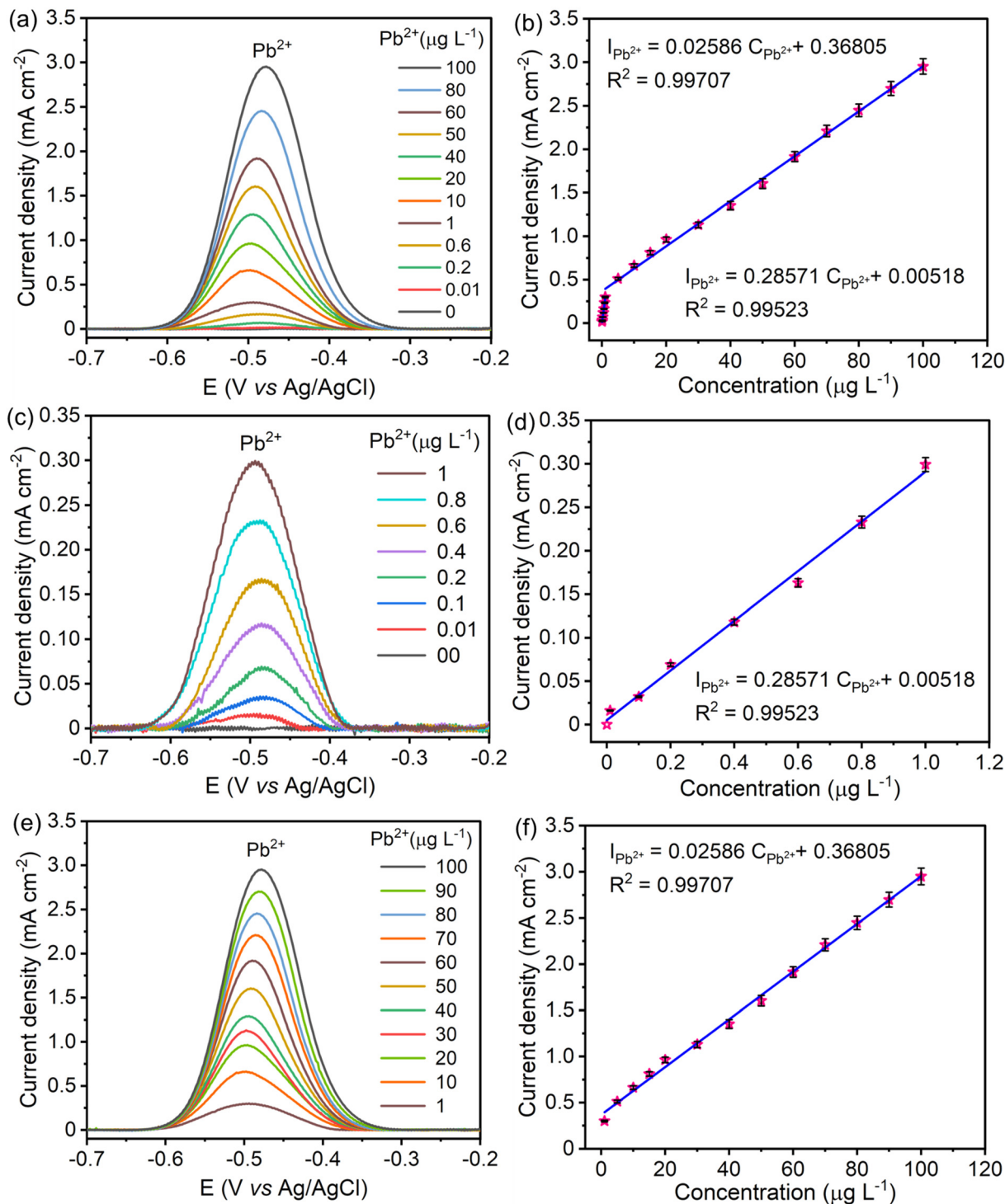
Fig. 8 SWASV responses of S-Bi@TiMX/PCE and the corresponding linear calibration plots of \text{Pb}^{2+} in 0.08 M \text{HClO}_4 solution, (a) and (b) 0.01 µg L -1 to 100 µg L -1 , (c) and (d) 0.01 µg L -1 to 1 µg L -1 , and (e) and (f) 1 µg L -1 to 100 µg L -1 \text{Pb}^{2+} .
