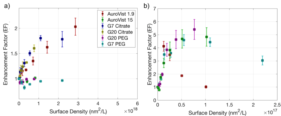
Fig. 7 EF of HO \cdot (a) and ^1\text{O}_2 (b) production under \gamma photon irradiation at doses of 0, 10 and 25 Gy for HO \cdot , and 0, 5 and 10 Gy for ^1\text{O}_2 , as a function of the AuNP surface density.
