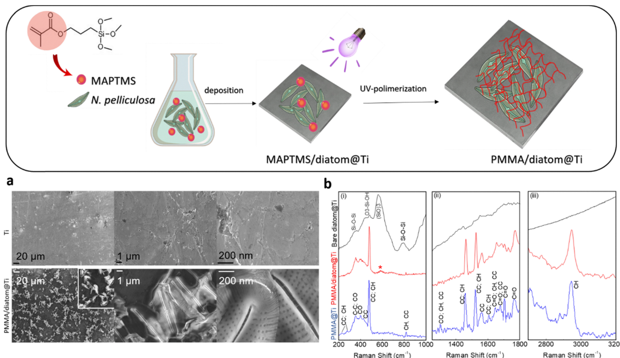
Fig. 1 Schematic representation of the preparation of PMMA/diatom@Ti scaffolds. (a) SEM images of the bare Ti (top) and PMMA/diatom@Ti (bottom) scaffolds. Scale bar: 20 μm, 1 μm and 200 nm. (b) Raman spectra of the bare diatoms (black line), PMMA/diatom@Ti (red line) and PMMA@Ti (blue line) in three different energy ranges (i) 200–1000 cm -1 , (ii) 1250–1800 cm -1 and (iii) 2700–3200 cm -1 . Specific chemical bonds are assigned to vibrational bands. Asterisk (*) indicates the presence of the (SiO) 3 bands in the spectrum of PMMA/diatom@Ti.
