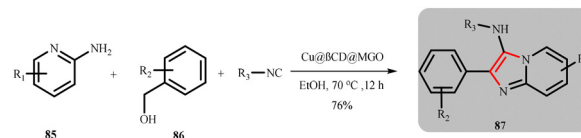
Scheme 40 Catalytic synthesis of N -(alkyl)-2-phenylimidazo[1,2- a ]pyridin-3-amine derivatives using \text{Cu}@\beta\text{-CD}@\text{MGO} nanoparticles (Bahadorikhalili et al. ).
