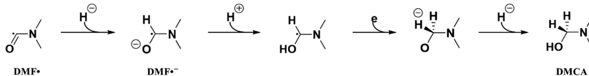
Fig. 5 Schematic of the DMCA preparation from DMF• generated by the DBD-catalyzed MOFs preparation in DBD liquid plasma. Reproduced from ref. 61 with permission from RSC, copyright 2019.
