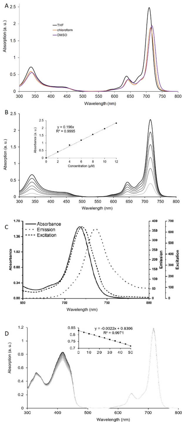
Fig. 1 (A) Superimposed UV-vis spectra of Pc2 in chloroform, DMSO and THF (10 \mu\text{M} ). (B) UV-vis absorption spectra of Pc2 in DMSO (2–12 \mu\text{M} ). Inset: Absorption vs. concentration. (C) Absorbance, emission (irradiation: 640 nm), and excitation spectra of Pc2 in DMSO. (D) Determination of singlet oxygen quantum yield of Pc2 in DMSO (6 \mu\text{M} ). Inset: Plot of DPBF absorbance at 417 nm vs. time.
