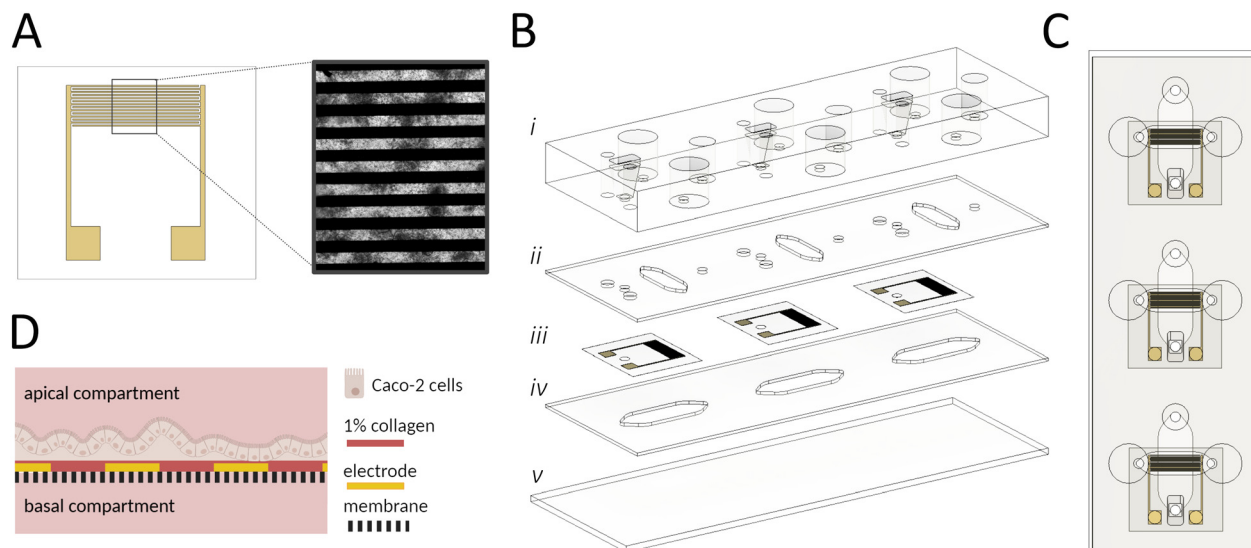
Scheme 1 (A) The electrode design features a pair of 7 interdigitated gold rods; the microscope image (Caco-2 cells) demonstrates the optical accessibility of the device. (B) Exploded view of the sensor-integrated gut-on-a-chip system comprising (i) a cast PDMS layer providing a lid and medium reservoir, (ii) an apical channel, consisting of a 500 \mu\text{m} PDMS sheet that accommodates the intestinal cells, (iii) 3 gold-electrodes onto a porous PET membrane, (iv) a 500 \mu\text{m} PDMS layer, serving as a basal compartment and (v) a microscope slide. (C) Top view of the platform emphasizes the 3 individual cultivation channels and the electrode (yellow) position aligned to the apical channel. (D) Schematic cross-section of the apical and basal compartment with cells. The porous membrane is represented by the dashed line, gold rods are depicted in yellow, and rat tail collagen type I coating is illustrated in red. The illustration is created with https://BioRender.com .
