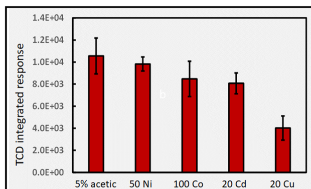
Fig. 15 Impact of added TMs (concentrations given as \mu\text{g mL}^{-1} ) on response (generation) of H_2 from photolysis of 5% (v/v) acetic acid at 2\text{ mL min}^{-1} (IT = 32 s; repeatability SD: n = 3 ). Uncorrected HS [ H_2 ] in 5% acetic acid is 270 \pm 40 ppm. Ordinate displays integrated response characterizing chromatographic peaks.
