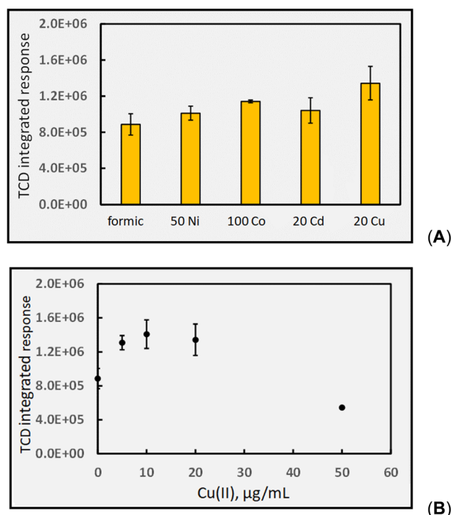
Fig. 9 Impact of added TMs (TM concentrations given as \mu\text{g mL}^{-1} ) on HS CO response (generation). Photolysis of 5% (v/v) formic acid at a solution flow rate of 2 mL min -1 (IT = 22 s). Ordinate displays integrated response characterizing chromatographic peaks. (A) Uncorrected HS [CO] increases from 4290 \pm 570 ppm to 6550 \pm 900 ppm (repeatability SD, n = 3 ) in the presence of 20 \mu\text{g mL}^{-1} Cu(II). (B) Effect of increasing Cu(II) on HS CO response (generation).
