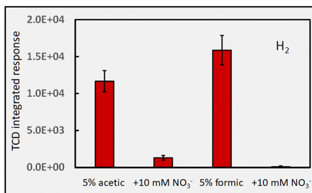
Fig. 8 Impact of the presence of 10 mM \text{NO}_3^- on HS \text{H}_2 response (generation) during photolysis of 5% (v/v) formic and acetic acids at 2 mL min -1 (IT = 22 s). Repeatability SD, n = 3 . Ordinate displays integrated response characterizing chromatographic peaks.
