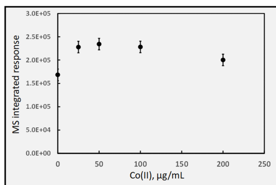
Fig. 14 (A) impact of added TMs (concentrations given as \mu\text{g mL}^{-1} ) on response (generation) of HS CO_2 during photolysis of 5% (v/v) acetic acid at 2\text{ mL min}^{-1} (IT = 32 s). Ordinate displays integrated response characterizing chromatographic peaks; (B) effect of added Co(II) on HS CO_2 response (generation). Uncorrected HS [ CO_2 ] increases from 1670 \pm 100 ppm to 2160 \pm 40 ppm (repeatability SD, n = 4 ) in the presence of 100\text{ }\mu\text{g mL}^{-1} Co(II).
